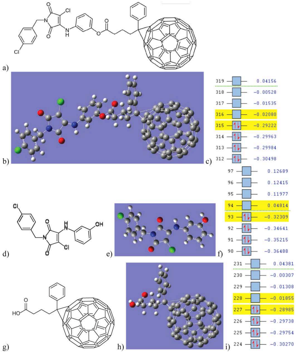
Fig. 1. (Color online) Structural-chemical formula (a) and spatial model (b) of C_{60} -MI nanocomplex based on [60]PCBA and 8335 KH. Gray balls represent carbon atoms, white ones are hydrogen, red ones are oxygen, green ones are chlorine, blue ones are nitrogen. (c) Energy values for the filled and unfilled molecular orbitals of the nanocomplex. Energy values are given in atomic units. (d)–(f) [60] 8335 KH compound, (g)–(i) [60]PCBA compound.
