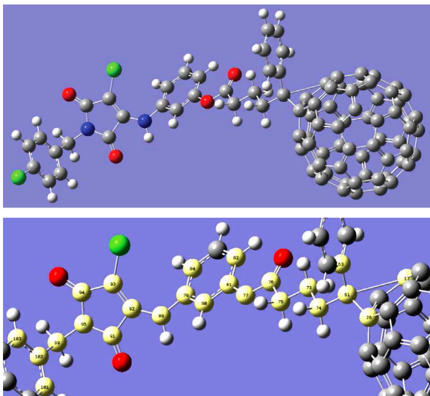
Fig. 5. (Color online) Angle 80_81_77 = 113.92, Angle 82_81_77 = 125.14, Angle 81_77_76 = 128.16, Angle 77_76_75 = 109.43; Angle 26_61_17 = 70.37, Angle 63_61_17 = 92.31, Angle 74_61_26 = 117.52, Angle 63_61_26 = 117.15, Angle 74_61_17 = 139.77, Angle 63_61_26 = 117.15.
