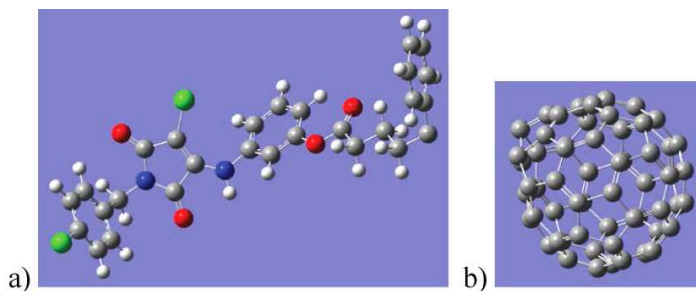
Fig. 4. (Color online) Spatial model: (a) “Linker”–“1H-pyrrole-2,5-dione”; (b) “C 60 -fullerene”. Gray balls represent carbon atoms, white ones are hydrogen, red ones are oxygen.
