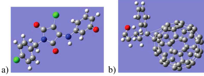
Fig. 2. (Color online) Spatial model: (a) “1H-pyrrole-2,5-dione”; (b) “C 60 -fullerene”–“Linker”. Gray balls represent carbon atoms, white ones are hydrogen, red ones are oxygen.
